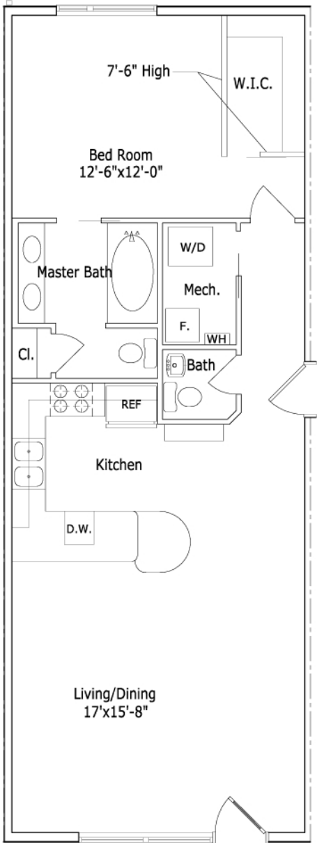
Ashe Ground Floor 1 bedroom 1.5 bath 860 s/f
